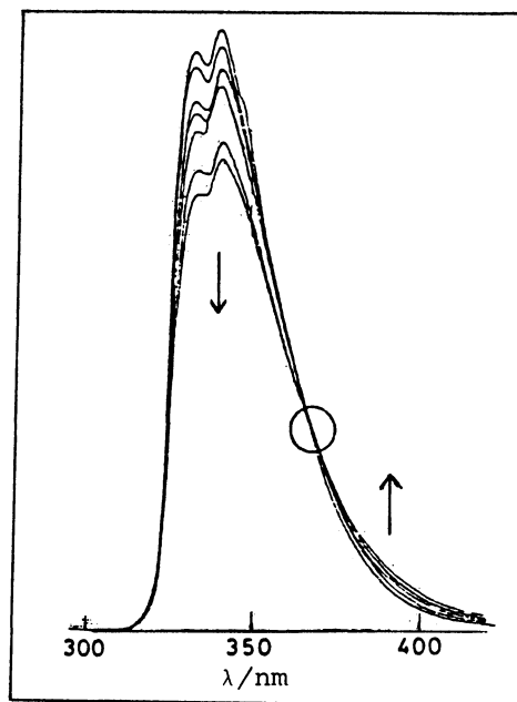
Fig. 1. Fluorescence spectra of CN in aerated benzene taken at different concentrations of 2; an isoemissive point is shown in the circle. The fluorescence quenching follows a linear Stern-Volmer plot with a slope of 4.5 \text{ dm}^3 \text{ mol}^{-1} .
